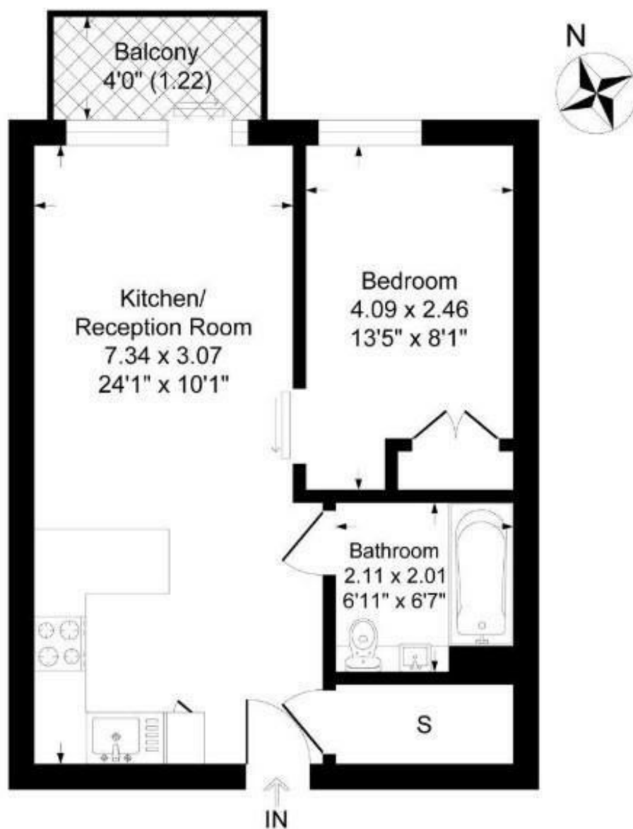
Second Floor
